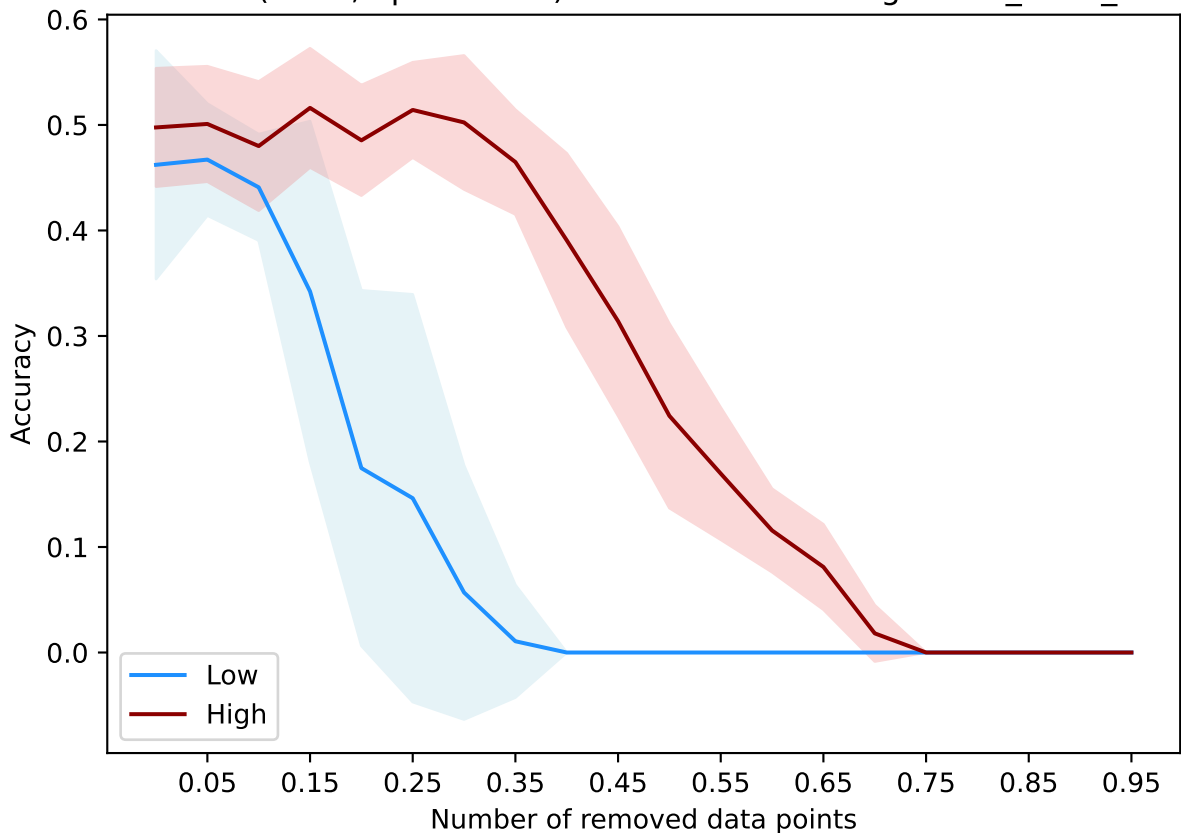
DataOob(1000, epochs=15) - cifar10-embeddingsworst_class_acc
